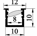
SJ-ALP1210-30D
