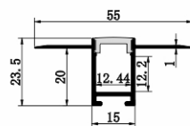
SJ-ALP5524-FLEX
