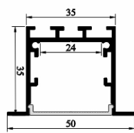
SJ-ALP3535-R5
