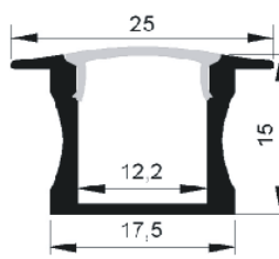
Dimension Drawing
