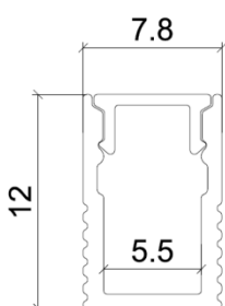
Aluminum Channel
